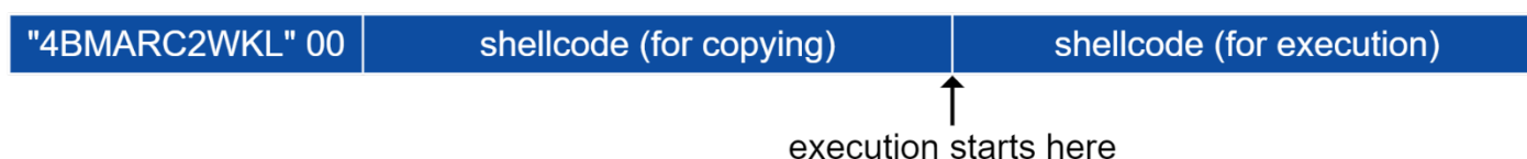
Fig. 2: Downloader shellcode buffer layout
